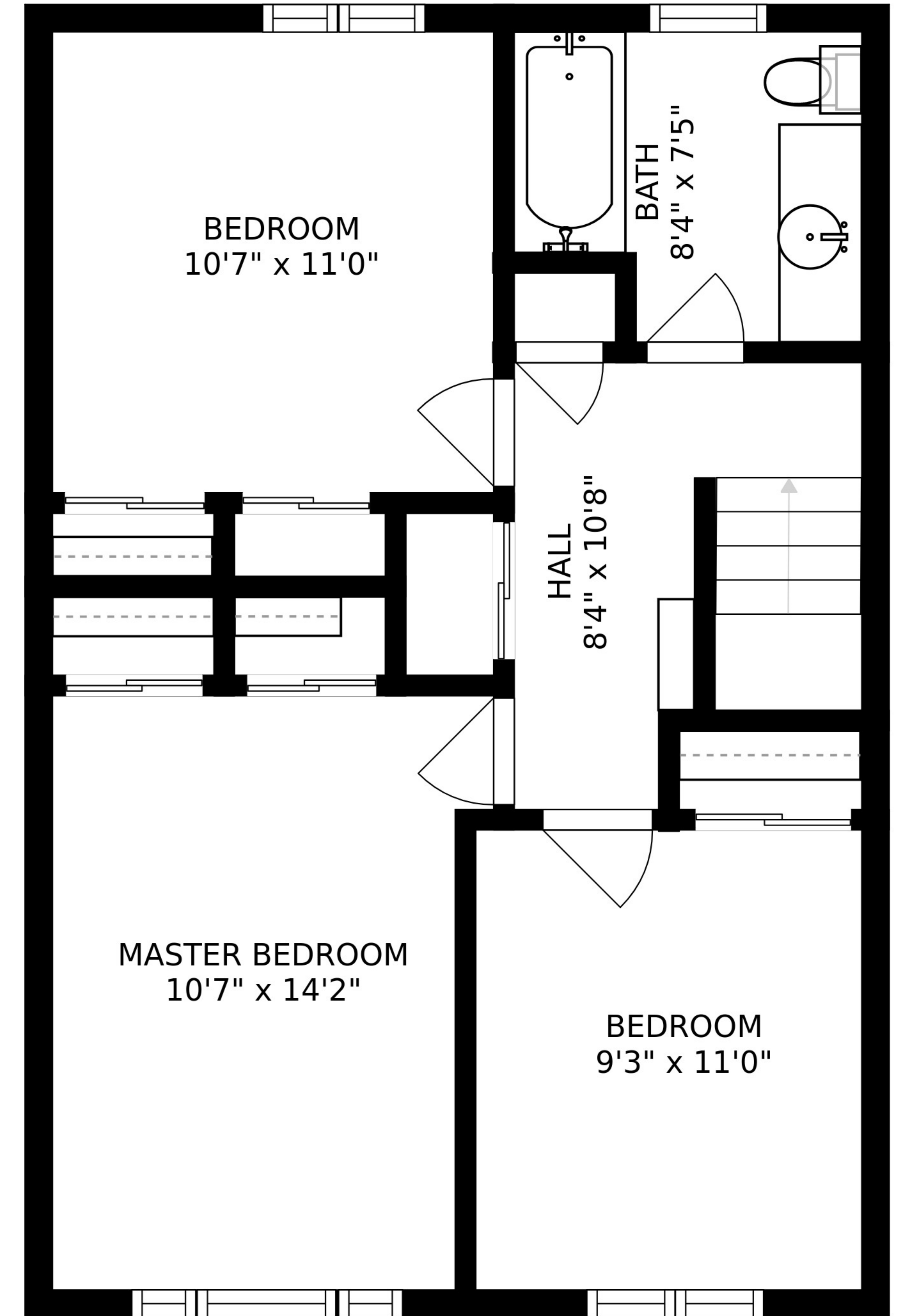
FLOOR 3
