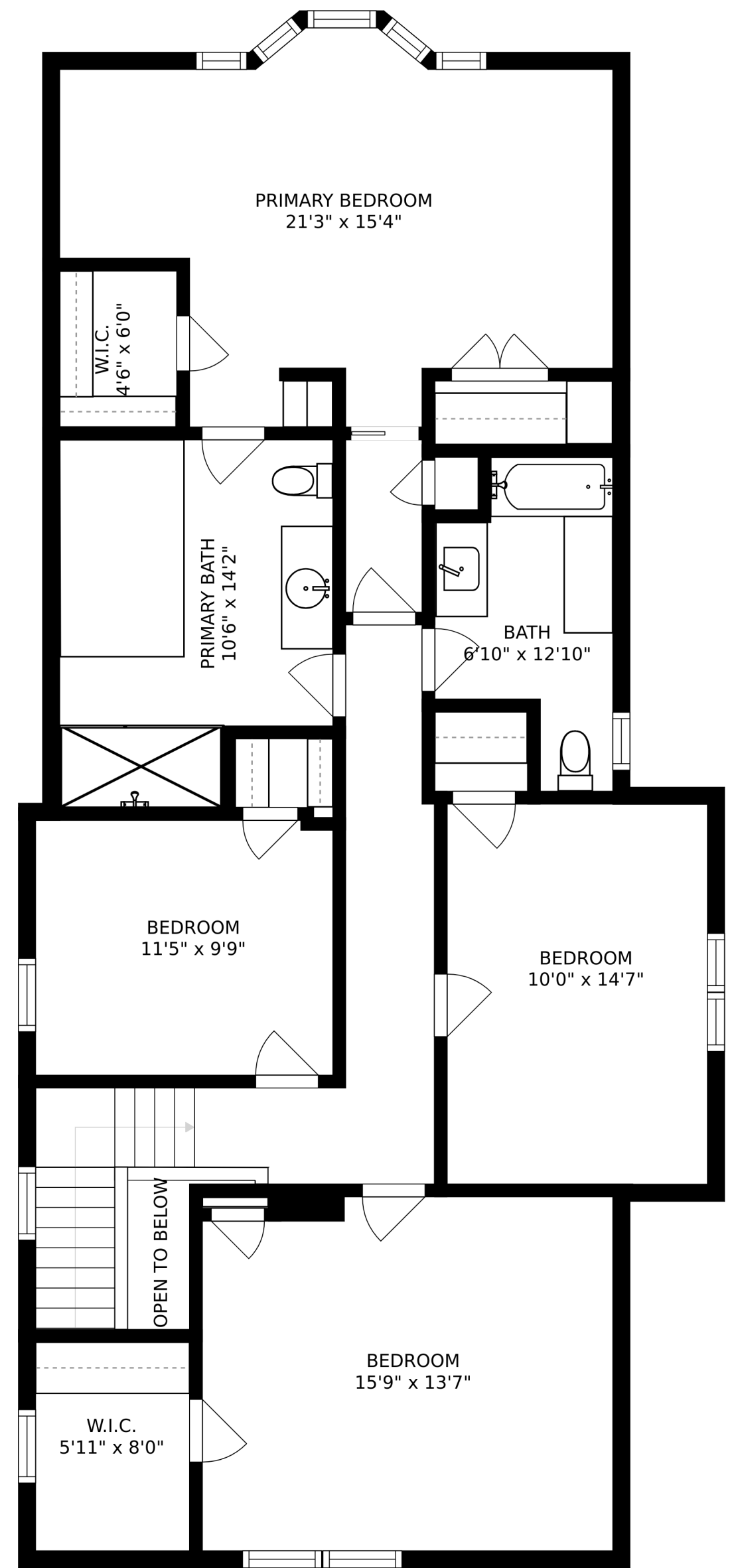
FLOOR 3
