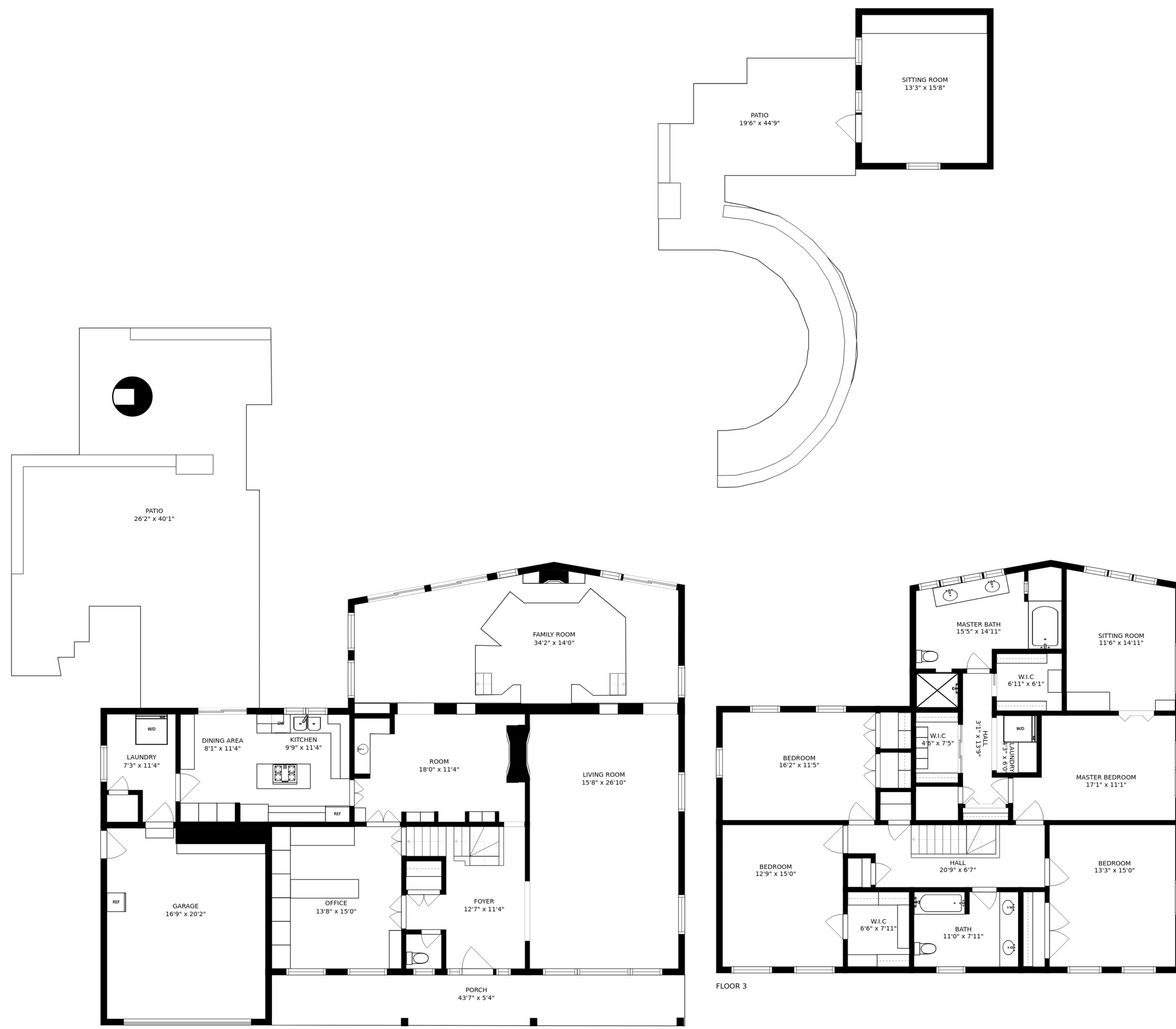
FLOOR 2
