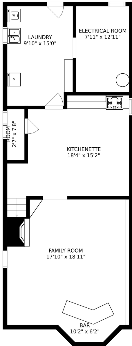
FLOOR 1
