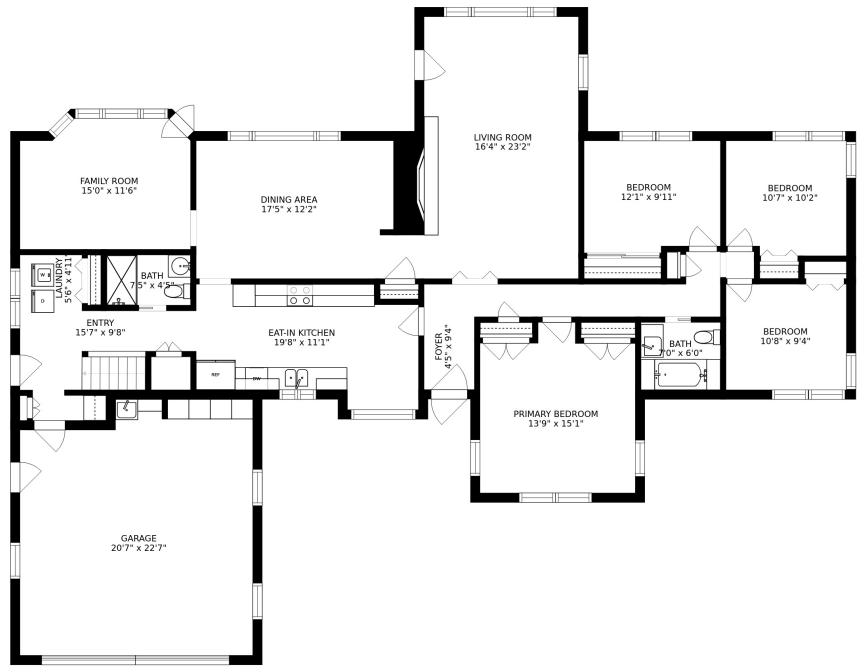
FLOOR 2
