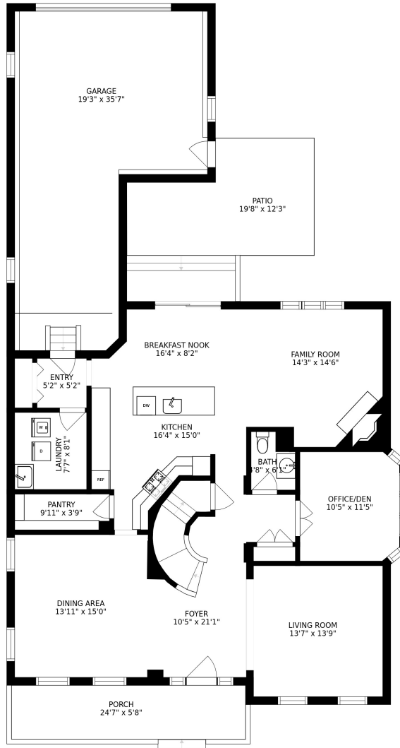
FLOOR 2
