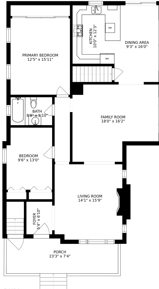
FLOOR 2
