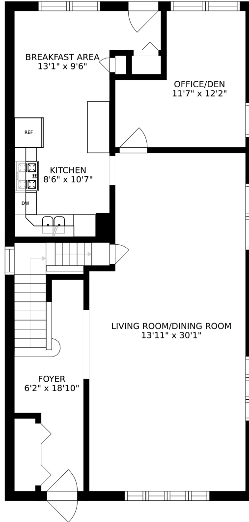
FLOOR 1
