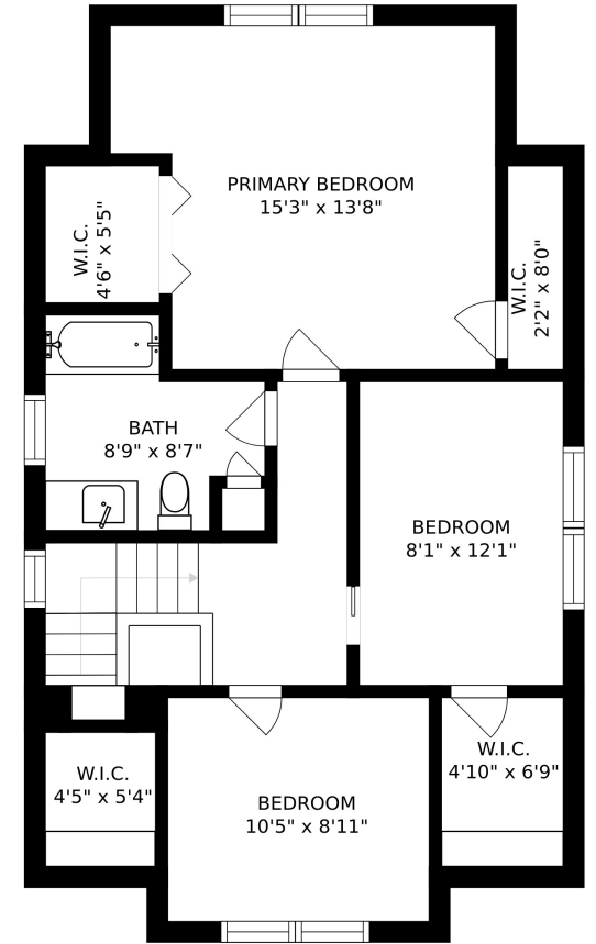
FLOOR 2
