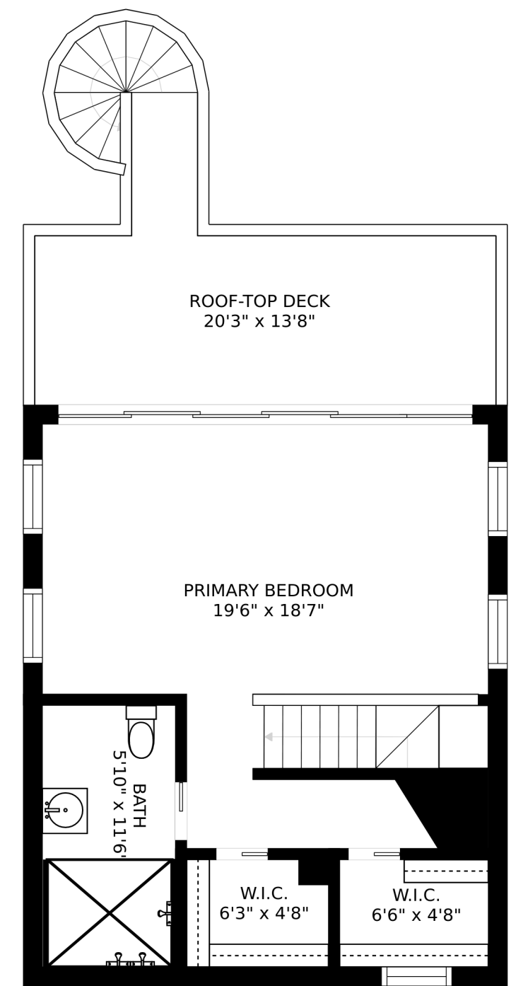
FLOOR 4
