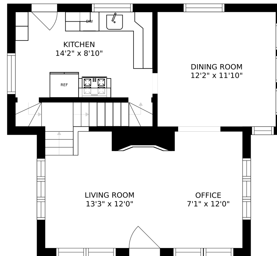
FLOOR 2
