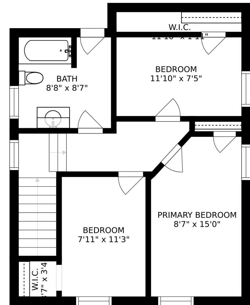
FLOOR 3
