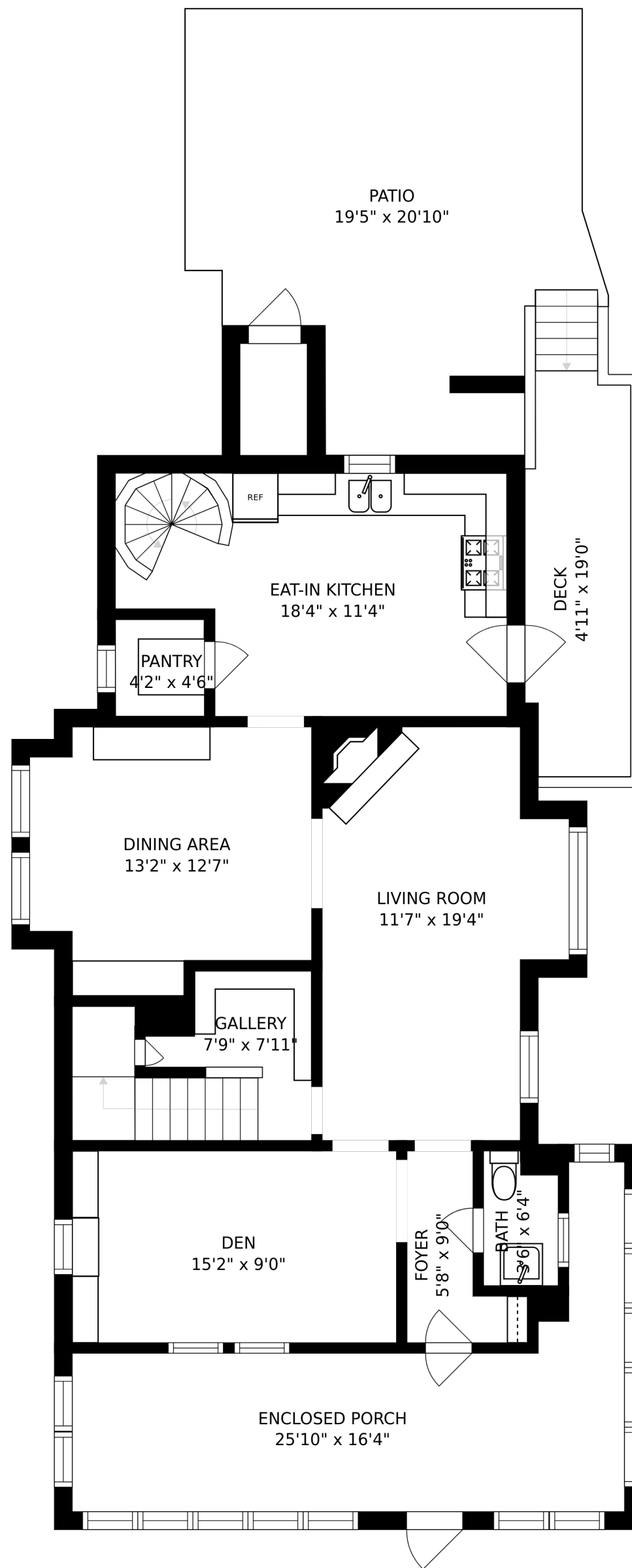
FLOOR 2
