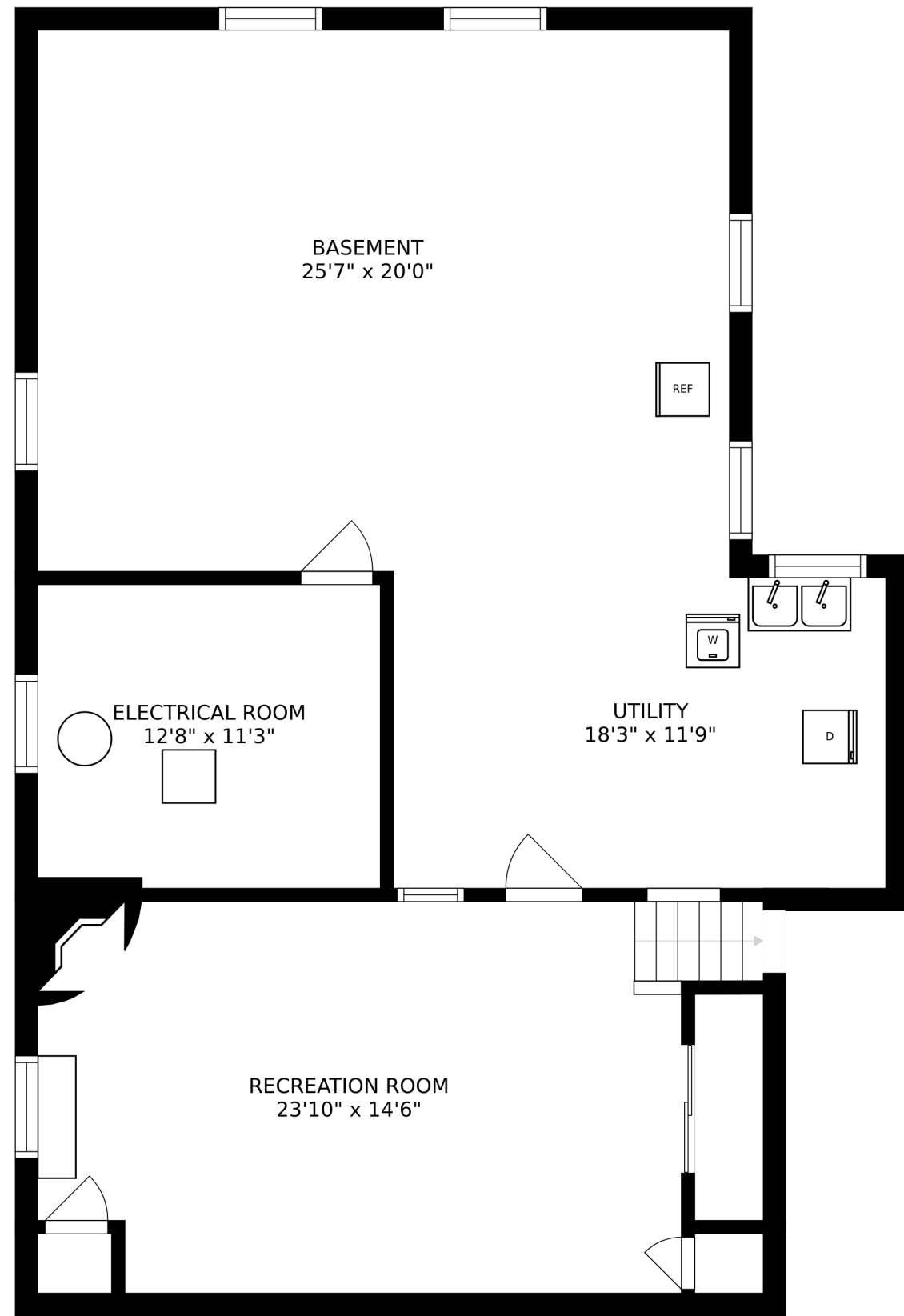
FLOOR 1
