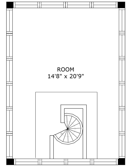
FLOOR 3
