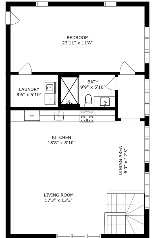
FLOOR 3
