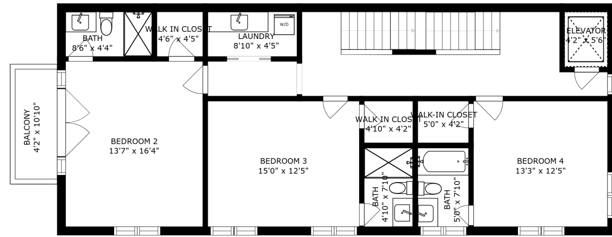
FLOOR 4
