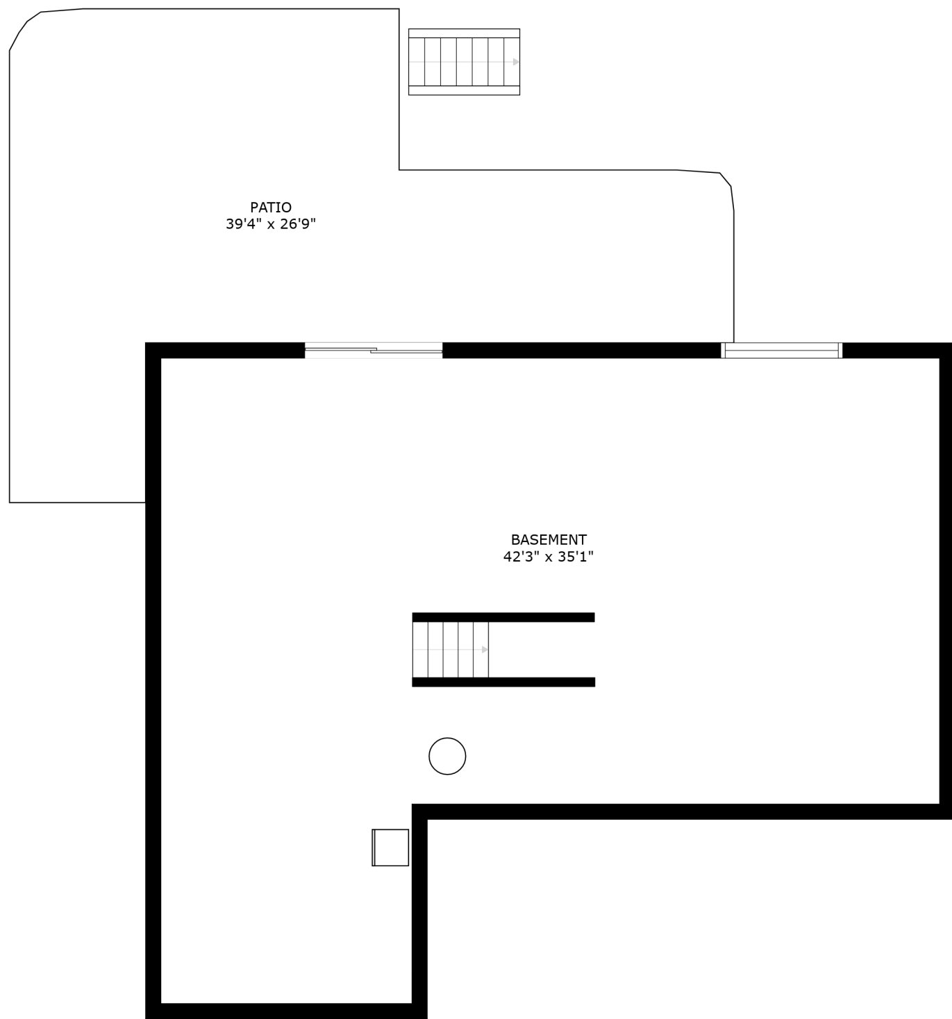
FLOOR 1
