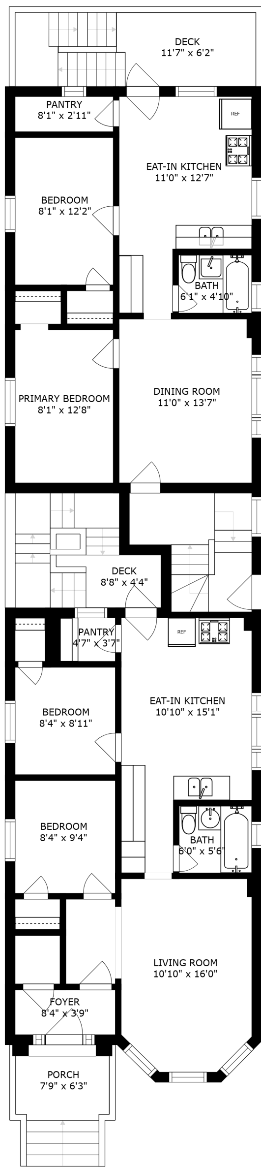
FLOOR 2
