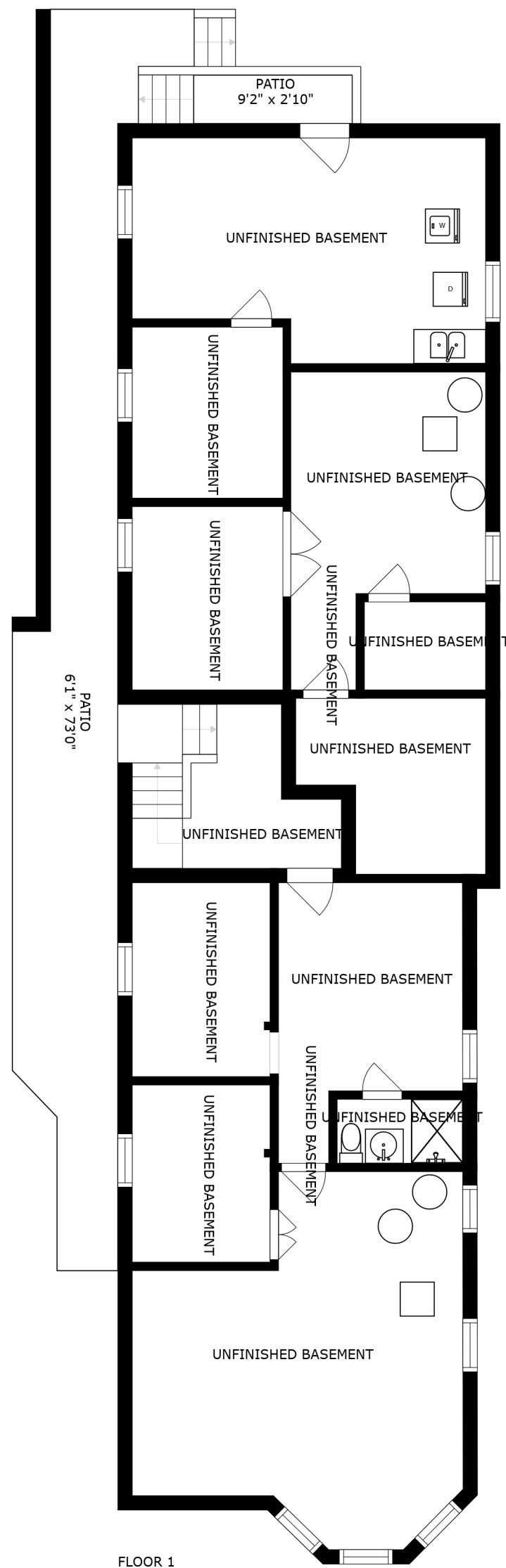
FLOOR 1
