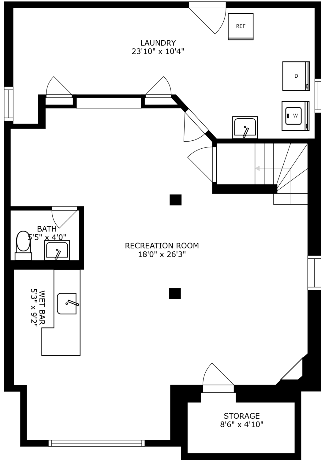
FLOOR 1
