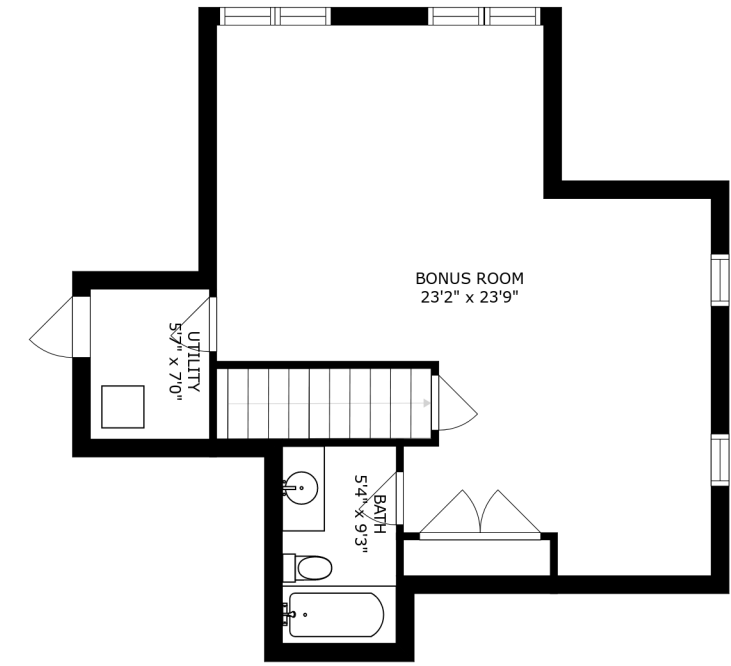
FLOOR 4
