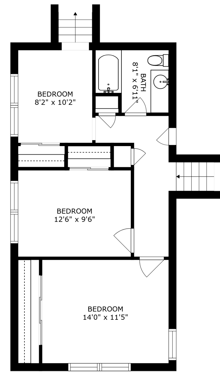
FLOOR 3
