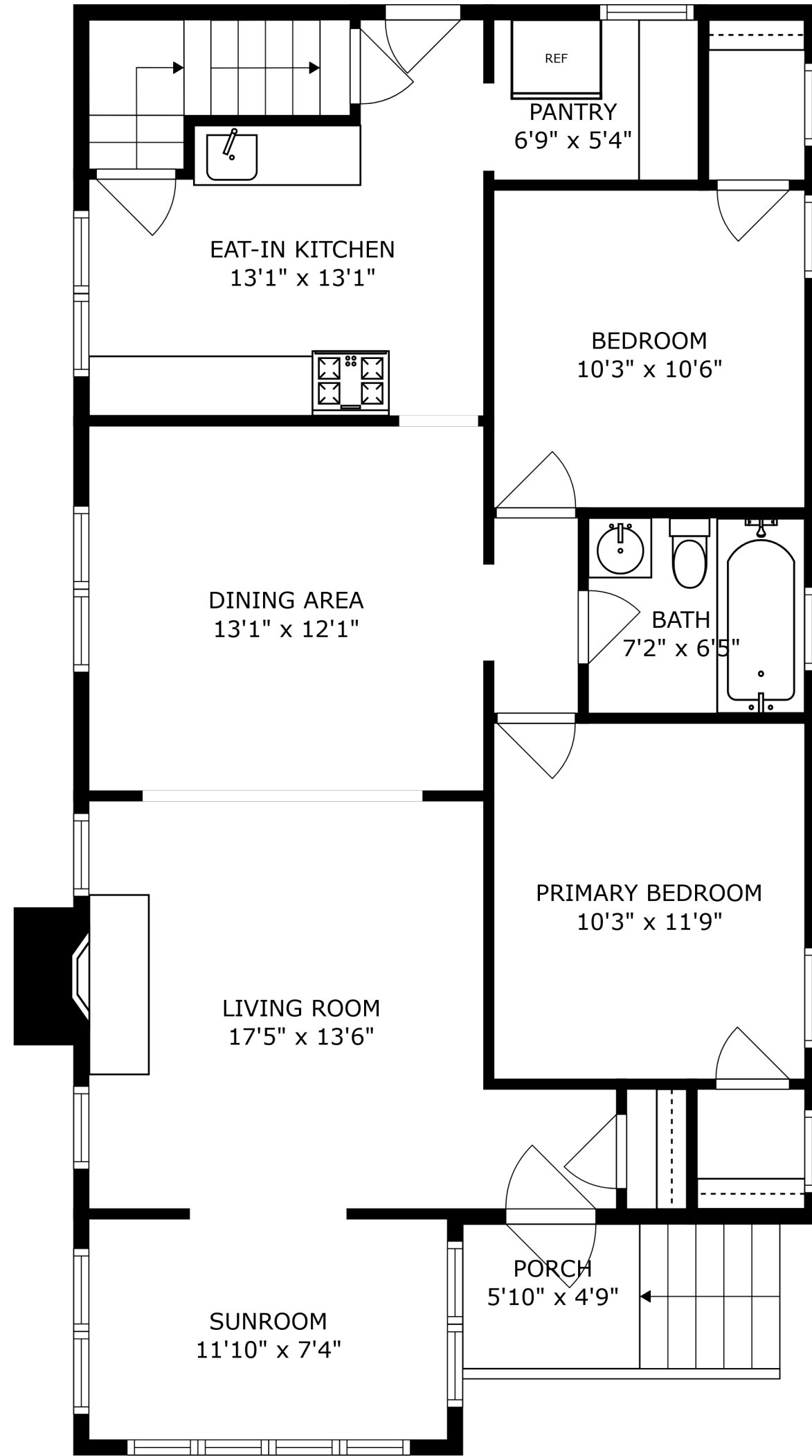
FLOOR 2
