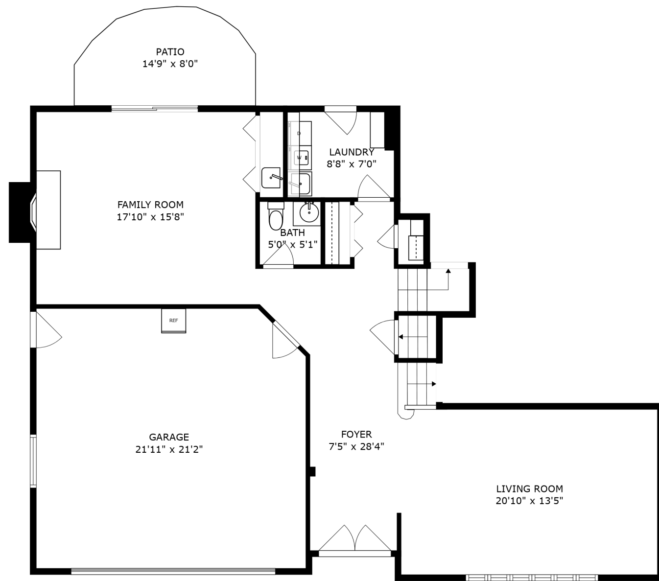
FLOOR 2
