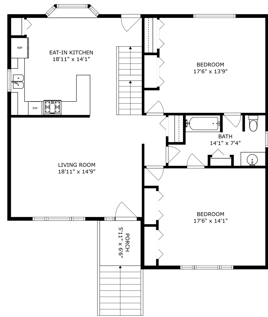
FLOOR 2
