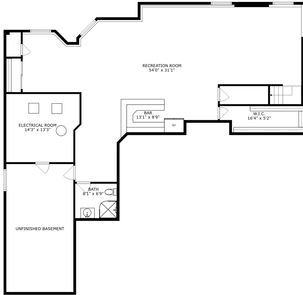
FLOOR 1
