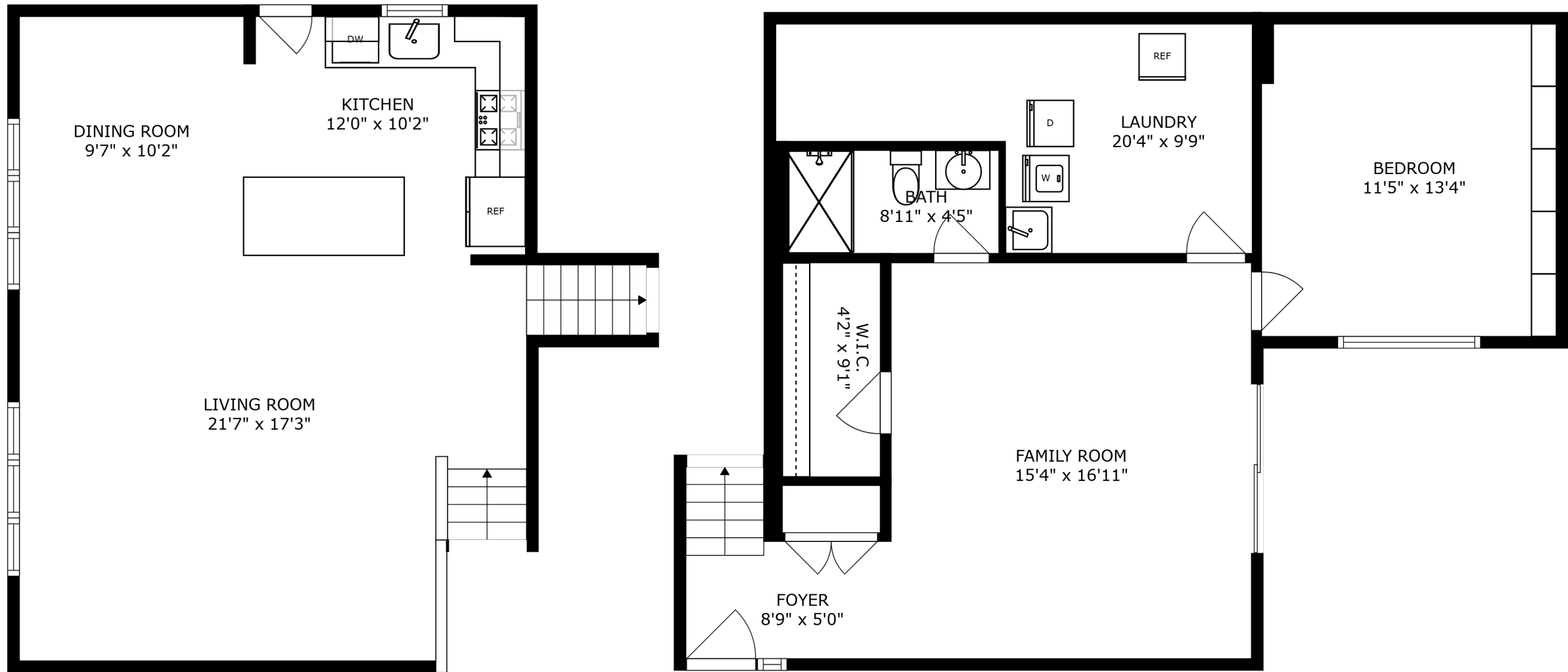
FLOOR 2
