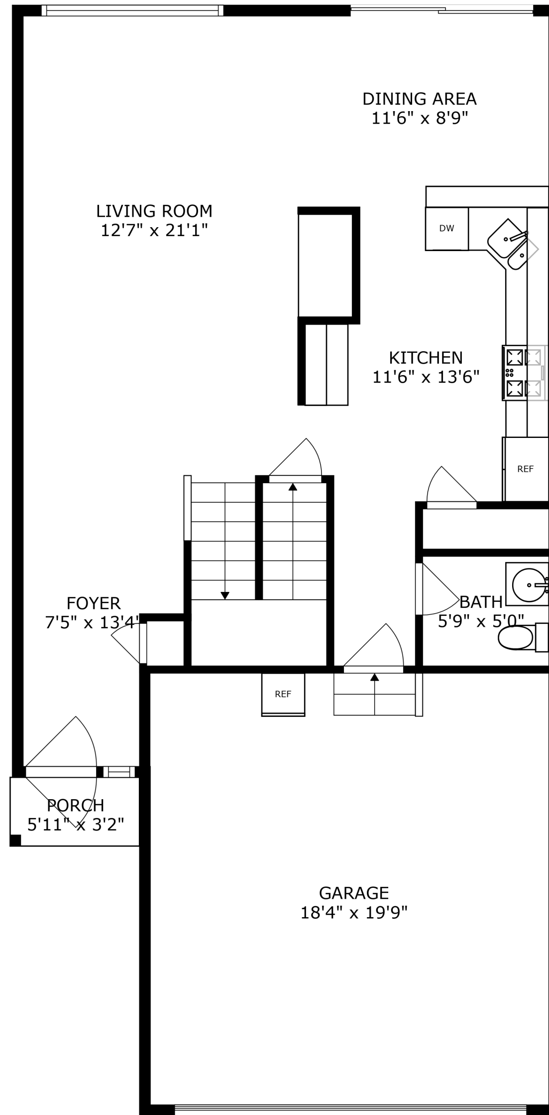
FLOOR 2
