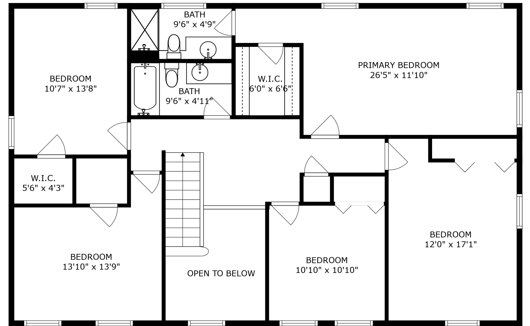
FLOOR 3
