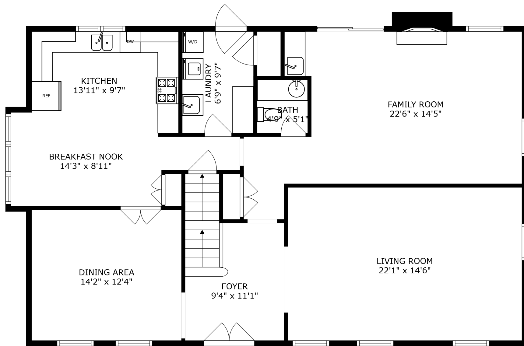
FLOOR 2
