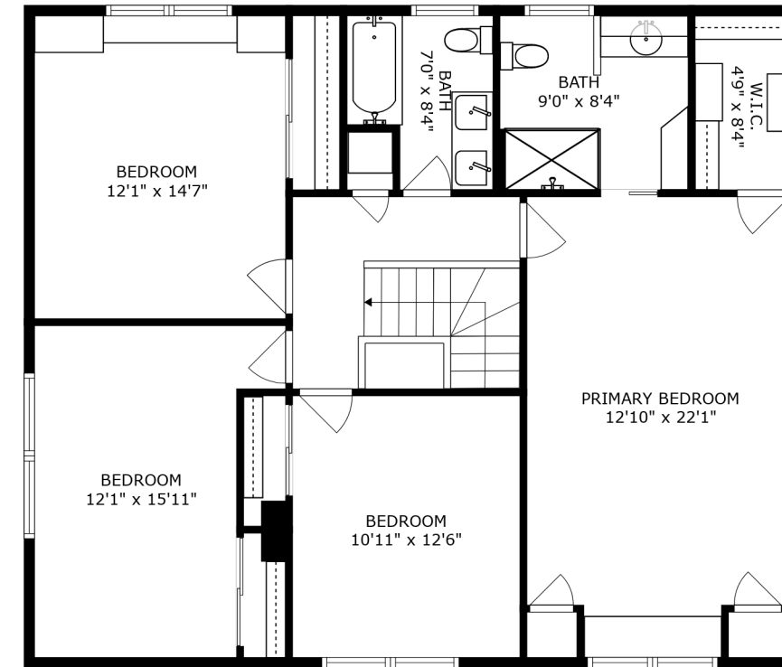
FLOOR 3
