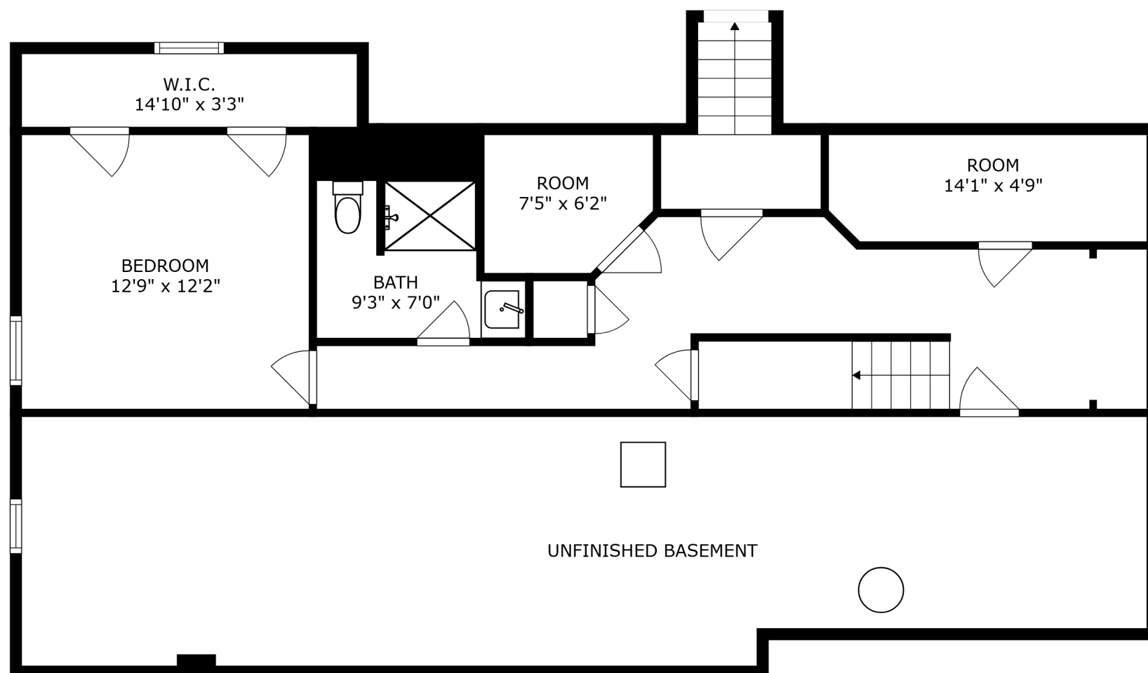
FLOOR 2
