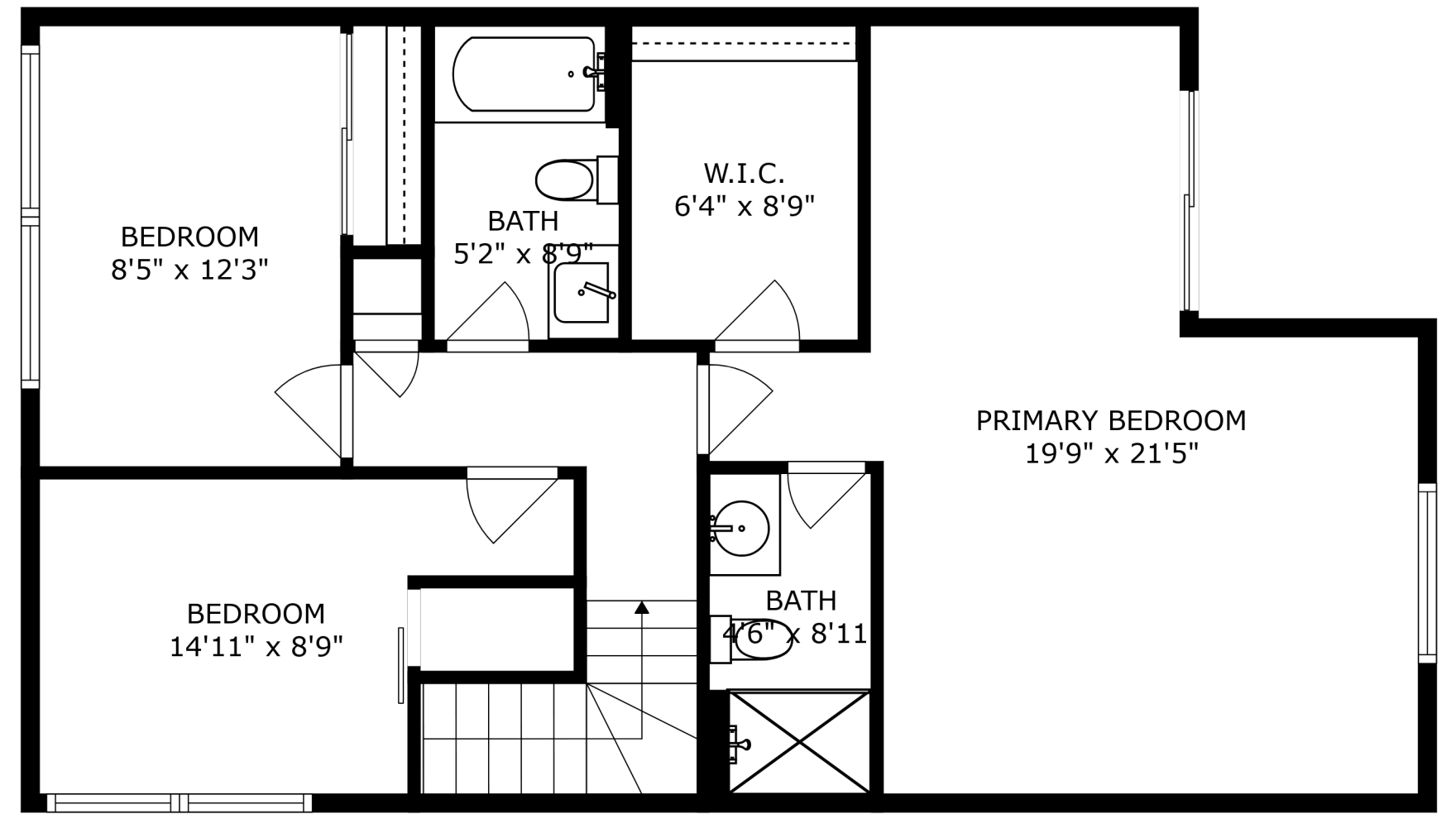
FLOOR 3
