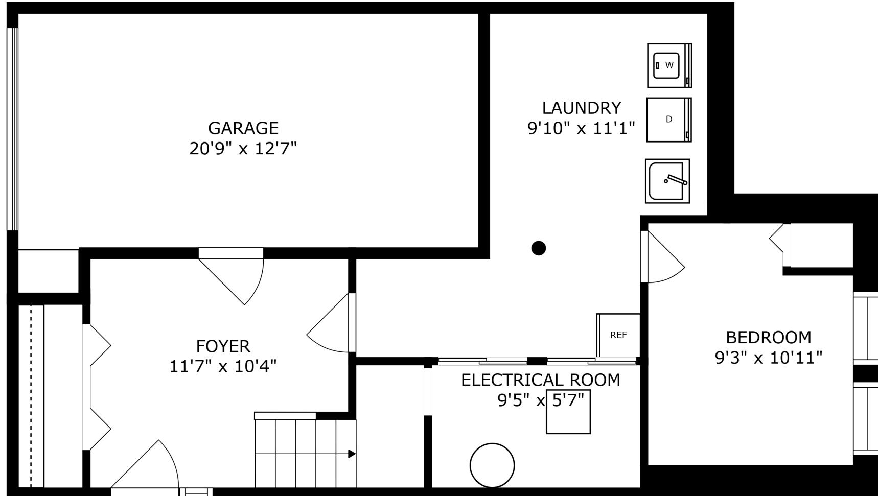
FLOOR 1
