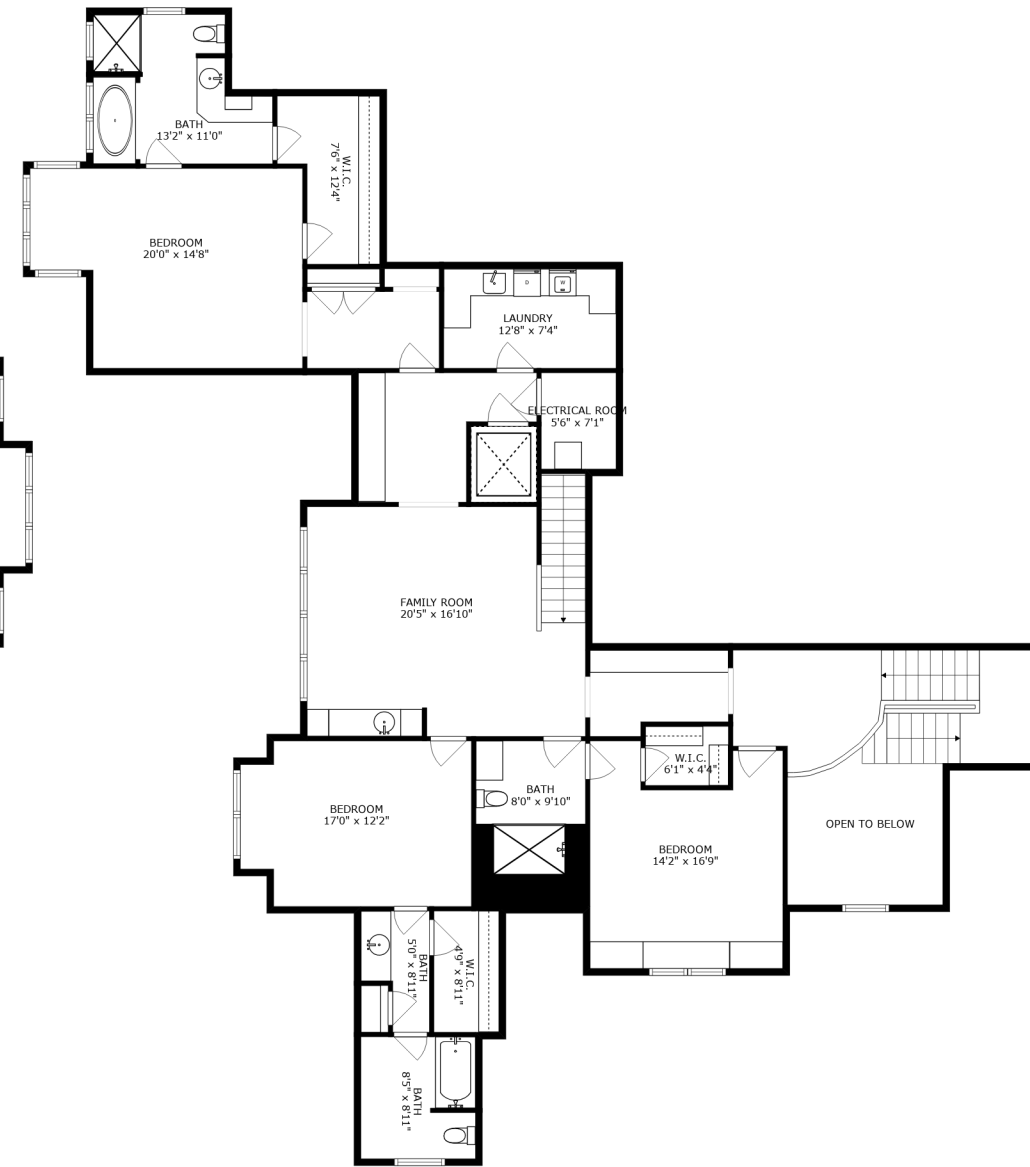
FLOOR 3
