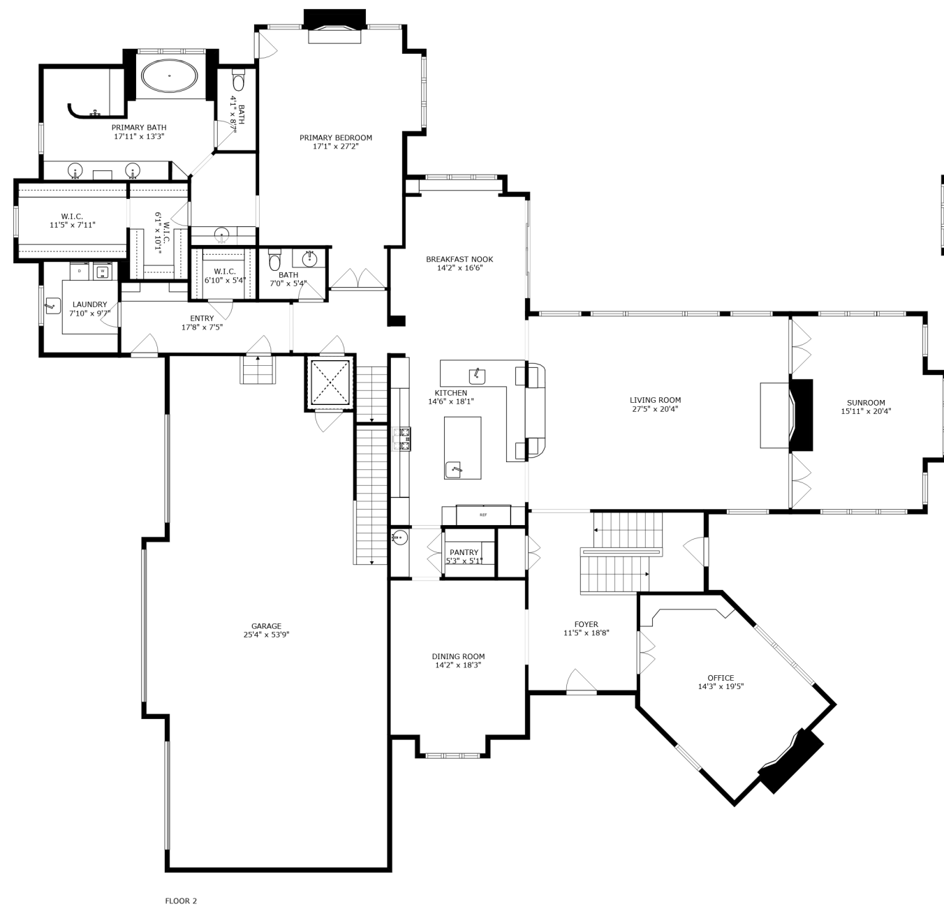
FLOOR 2
