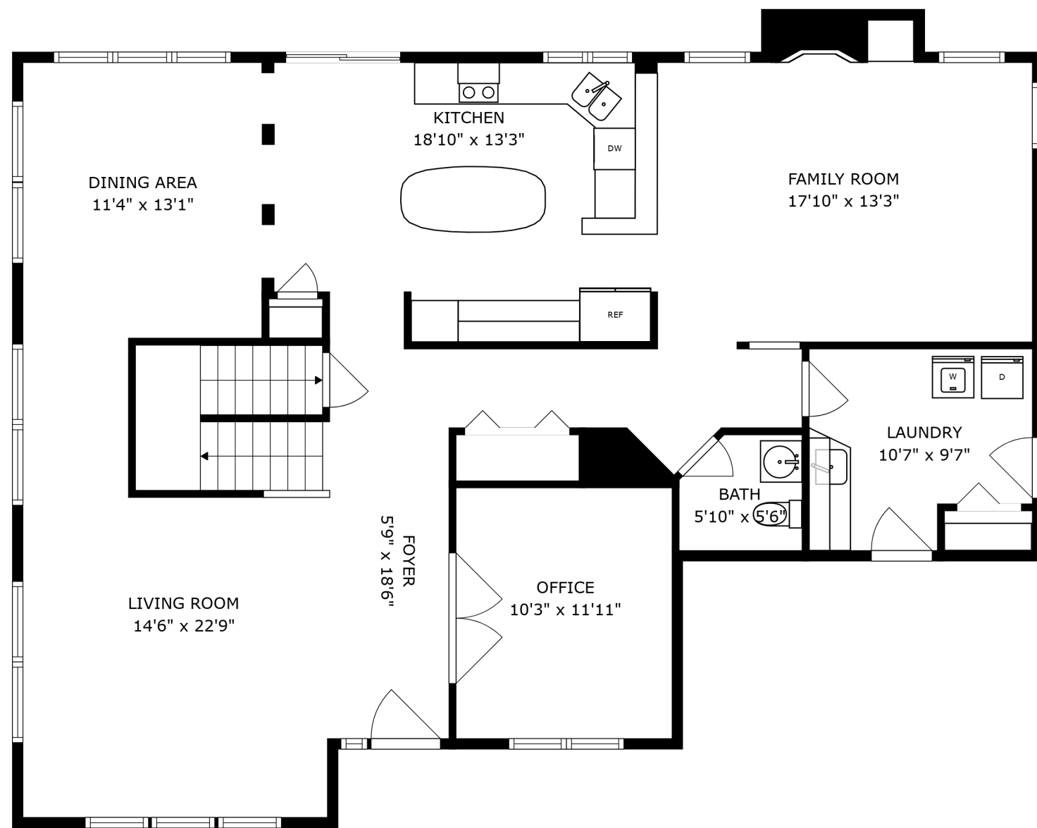
FLOOR 2
