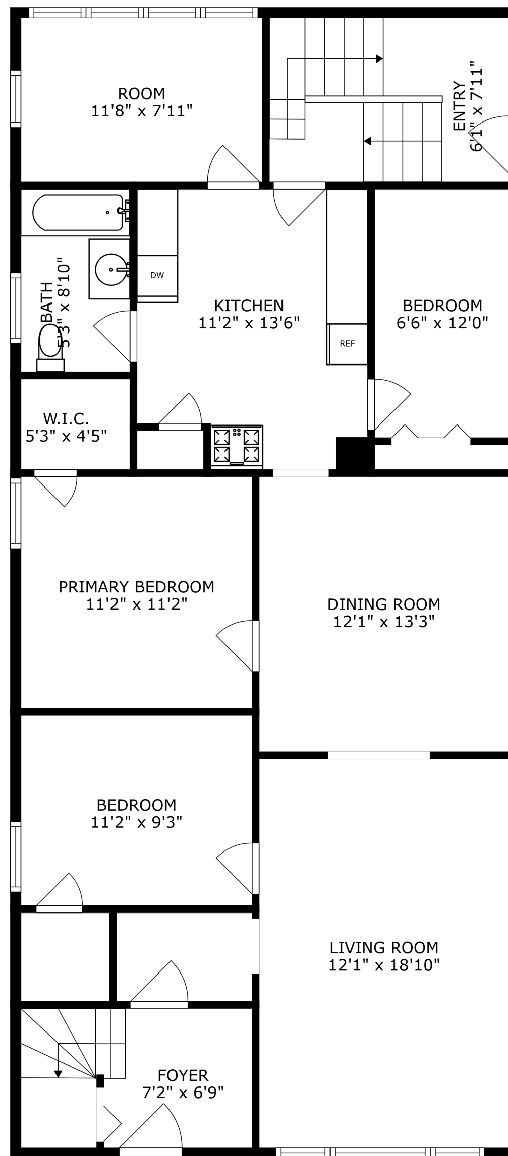
FLOOR 2
