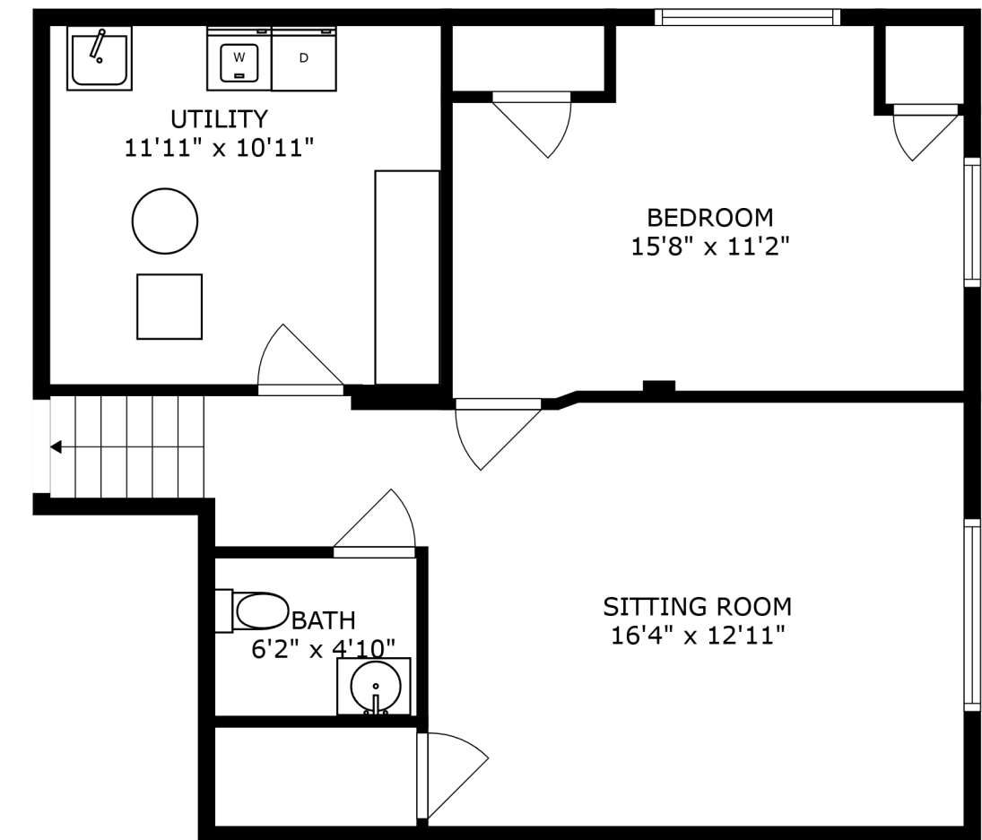
FLOOR 1
