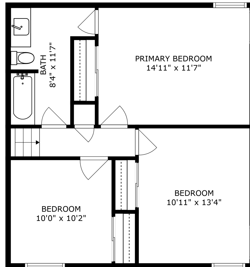
FLOOR 3
