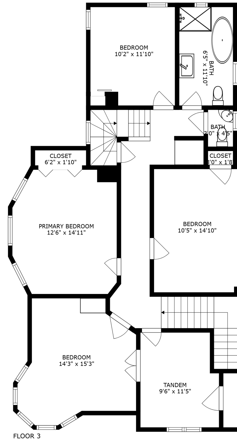
FLOOR 3
