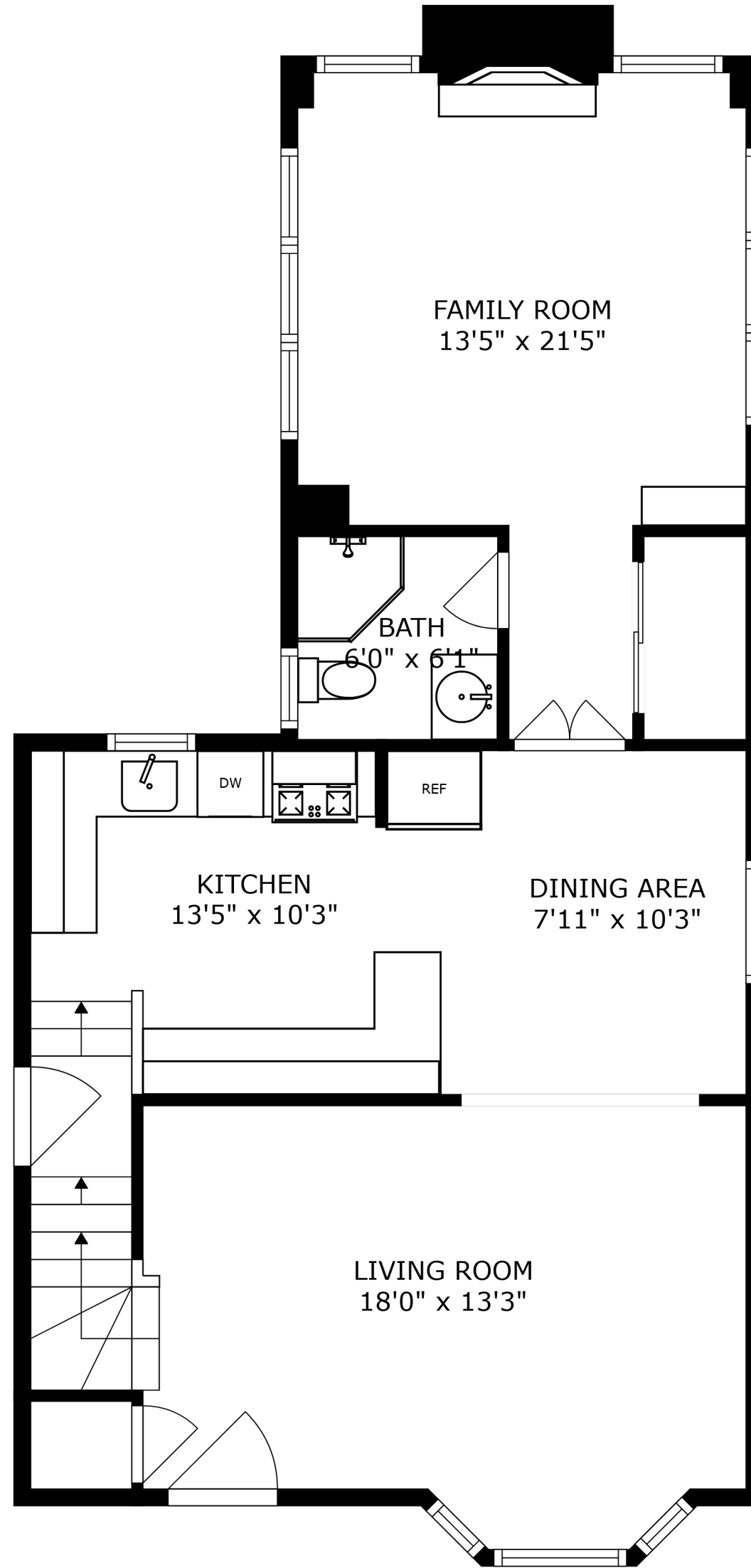
FLOOR 2
