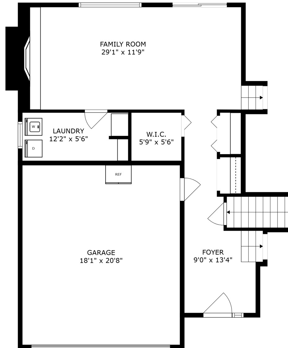
FLOOR 2
