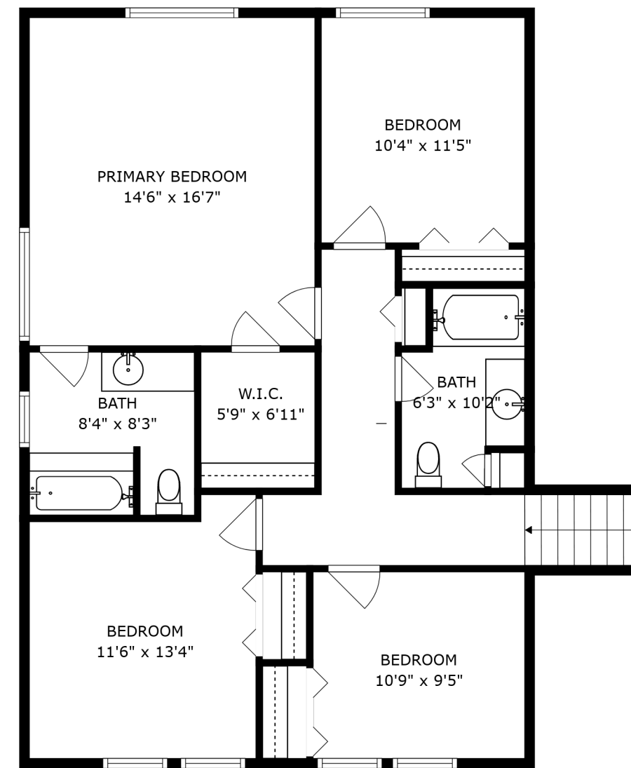
FLOOR 4
