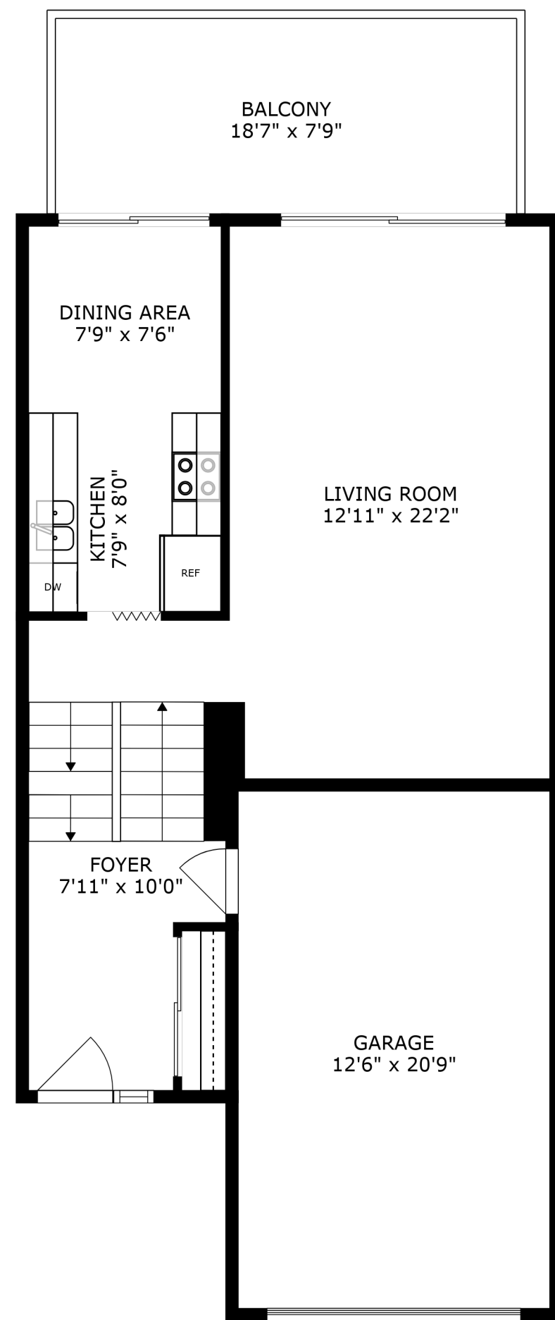
FLOOR 2
