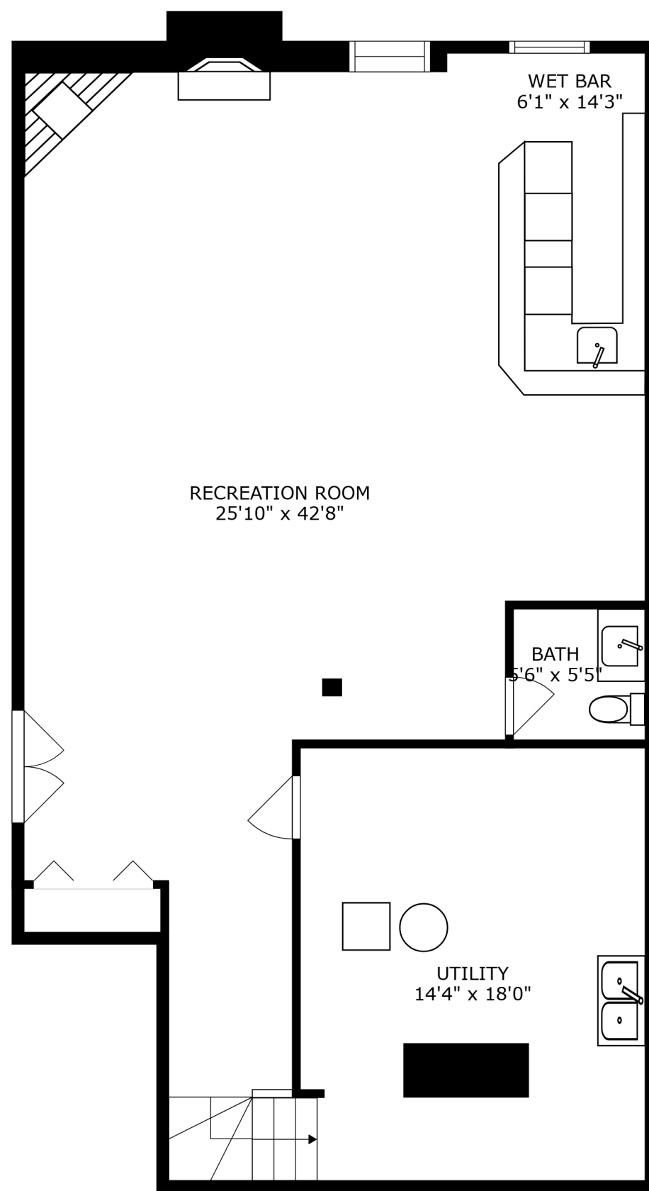
FLOOR 1
