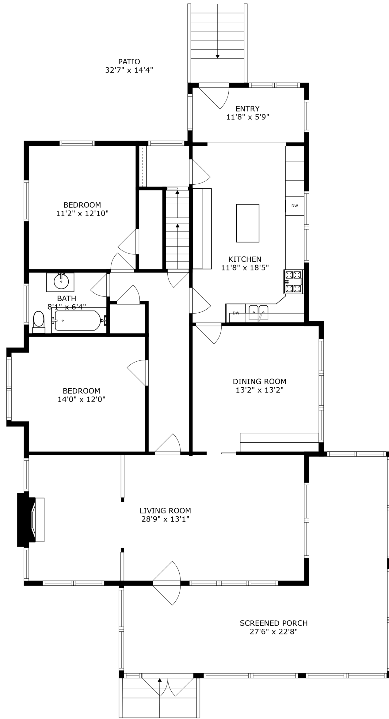
FLOOR 2
