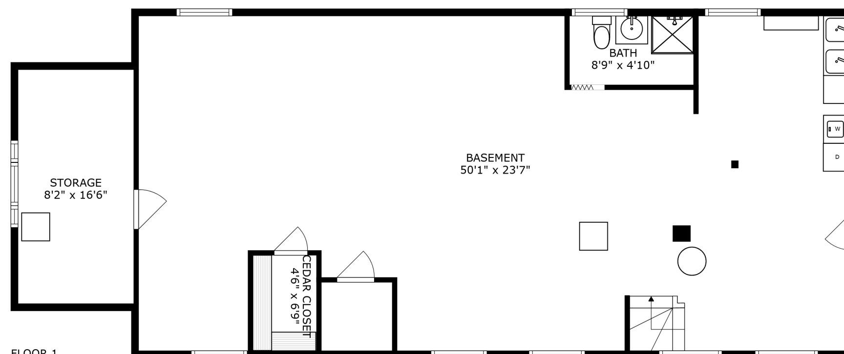
FLOOR 1
