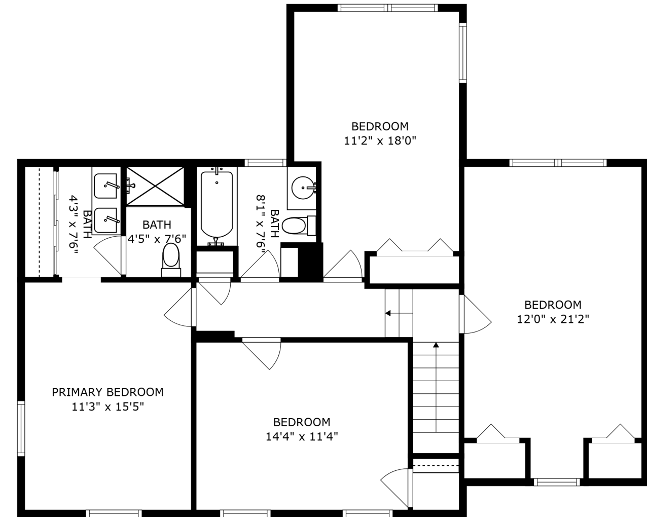
FLOOR 3
