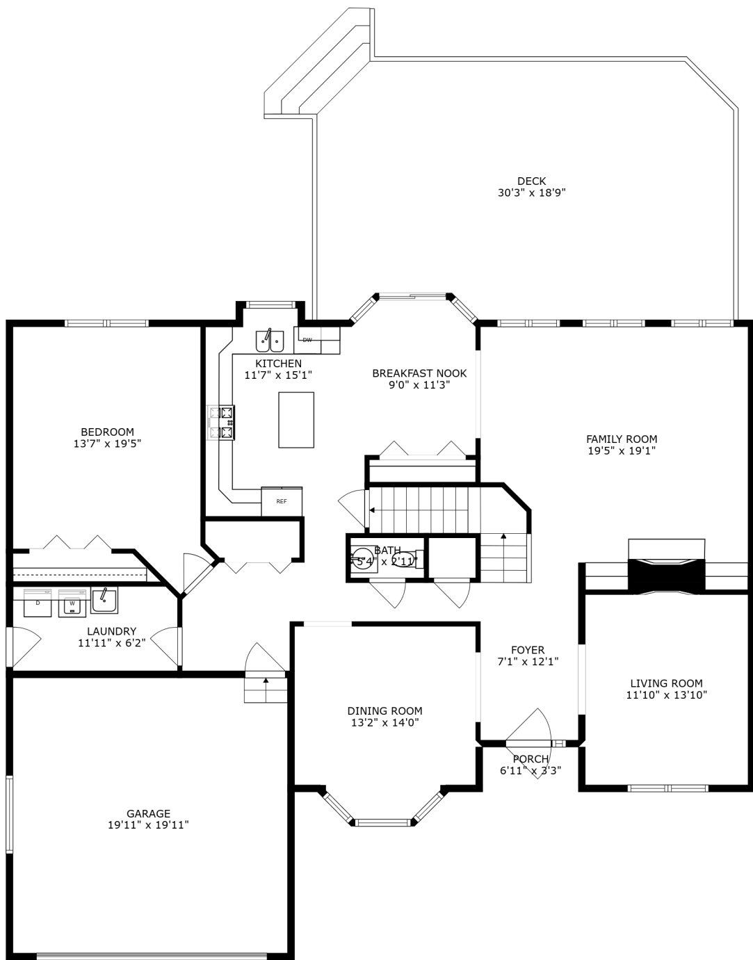
FLOOR 2
