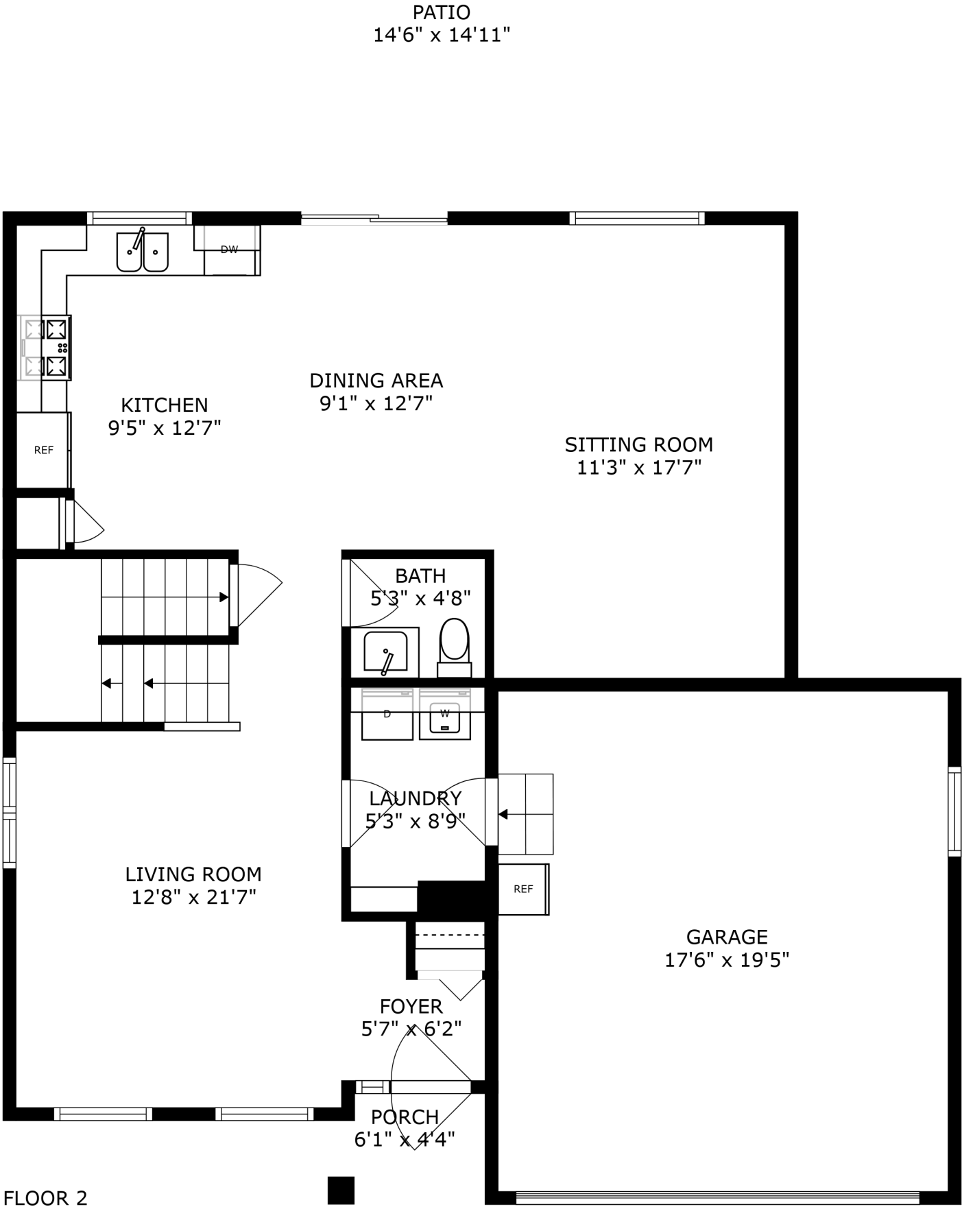
FLOOR 2
