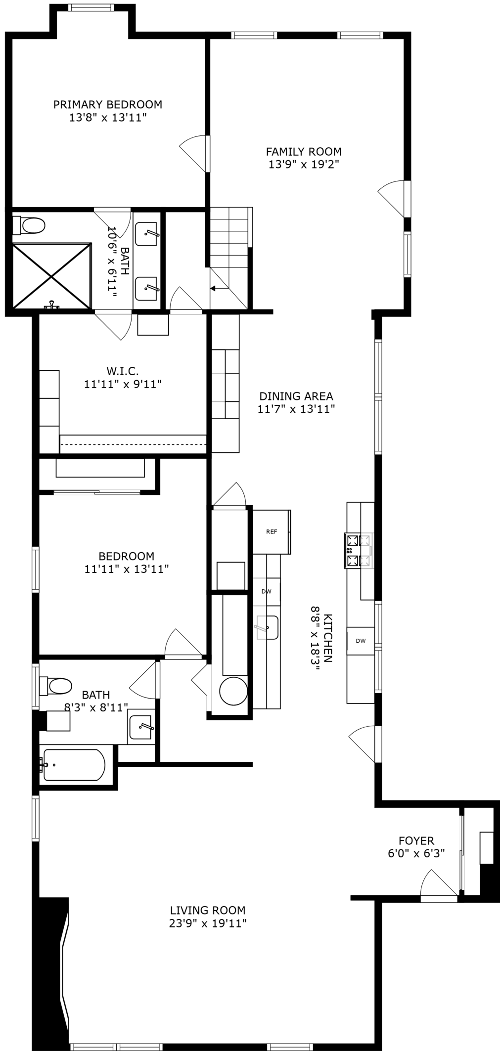
FLOOR 1
