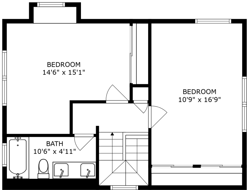
FLOOR 2
