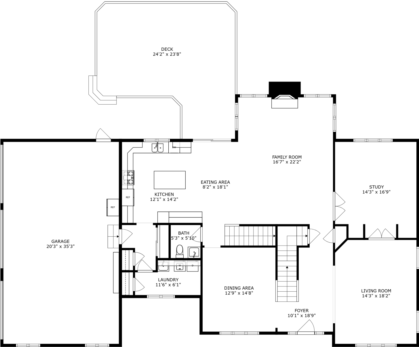
FLOOR 2
