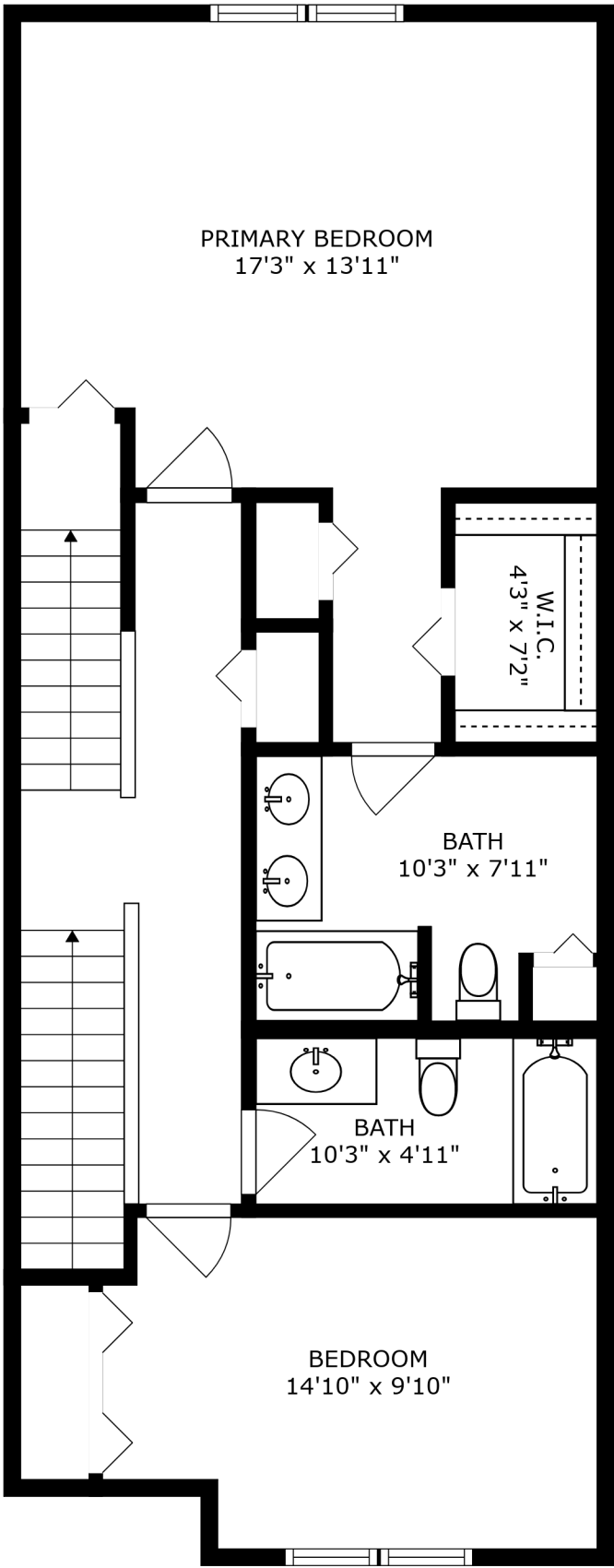
FLOOR 3
