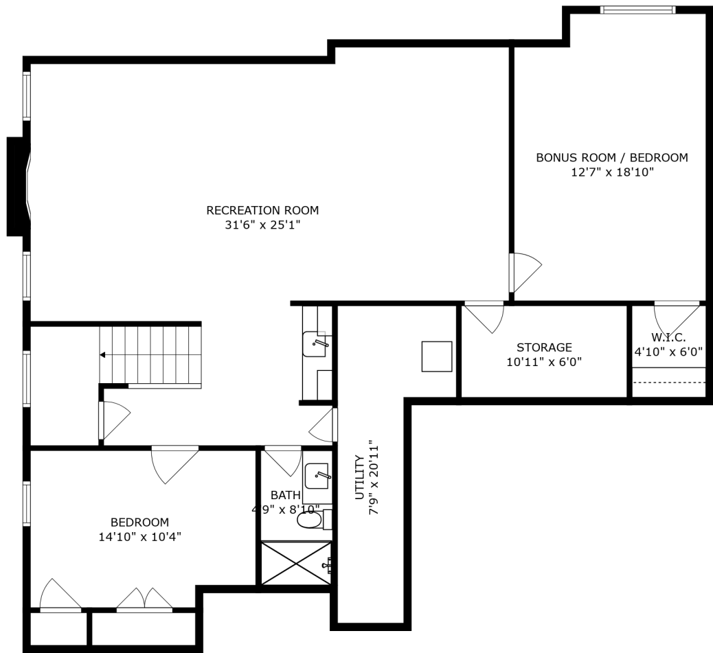
FLOOR 2
