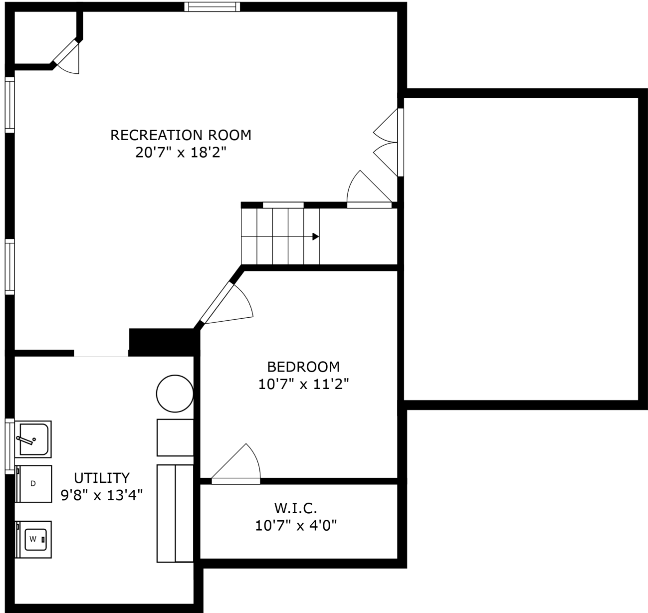
FLOOR 1
